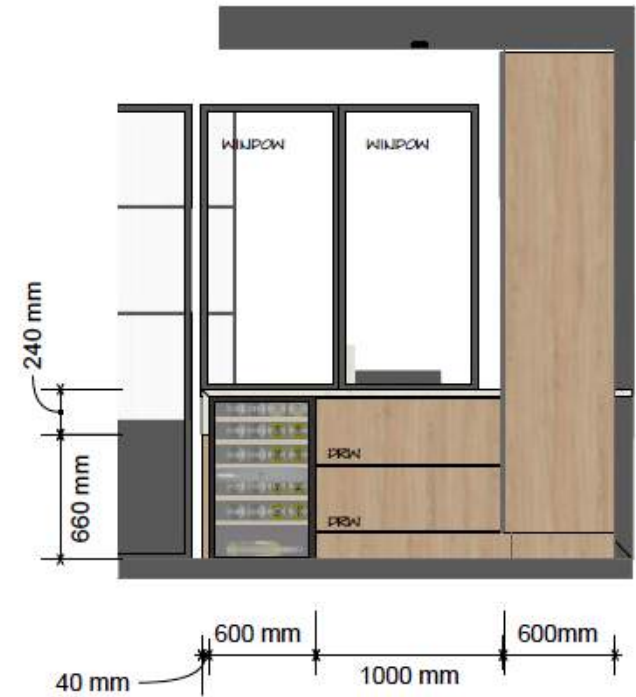
F SECTION F 1:40 @ A3
