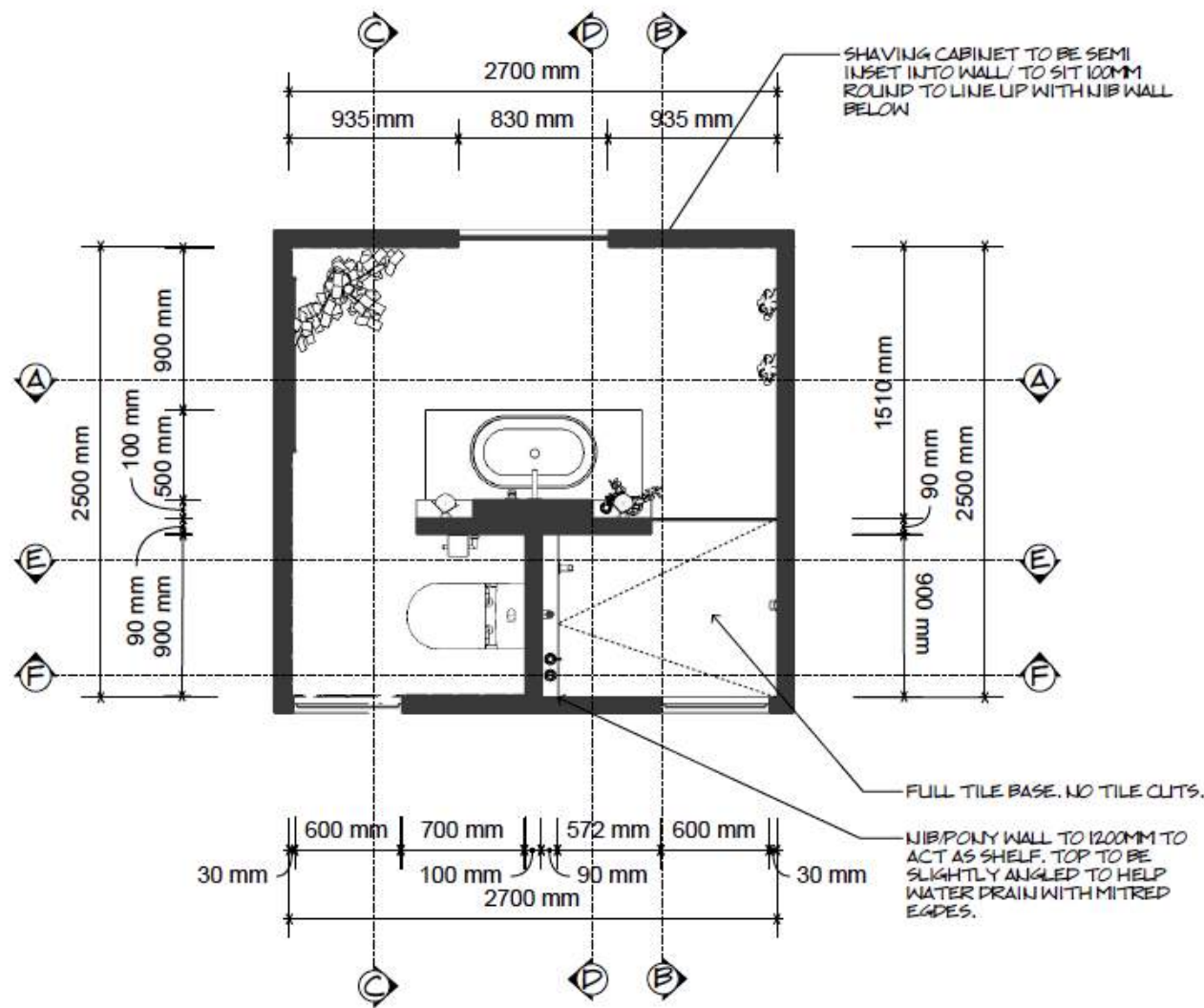
FLOOR PLAN 1:40 @ A3
