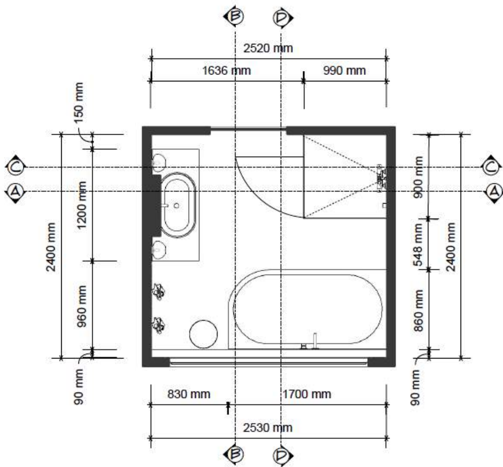
FLOOR PLAN 1:40 @ A3
