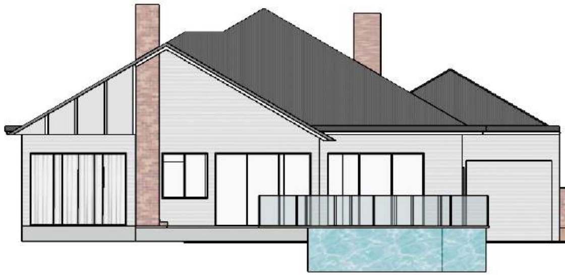
N NORTHERN ELEVATION 1:125 @ A3
